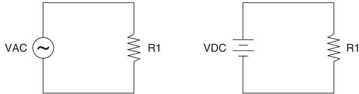
(Power consumed in R1 is same for both AC & DC source if the VAC RMS equals VDC)
